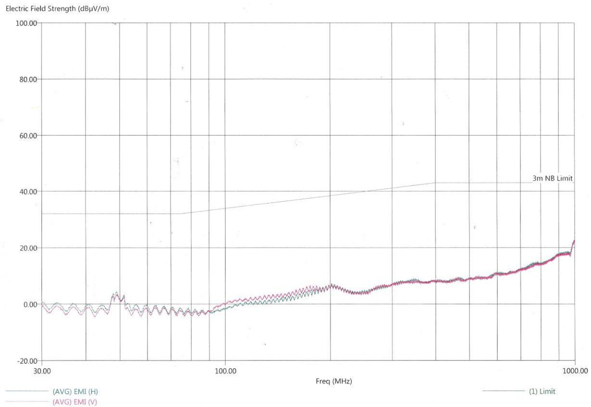
Fig.: EMC measurement of turntable with integrated dynamometer
